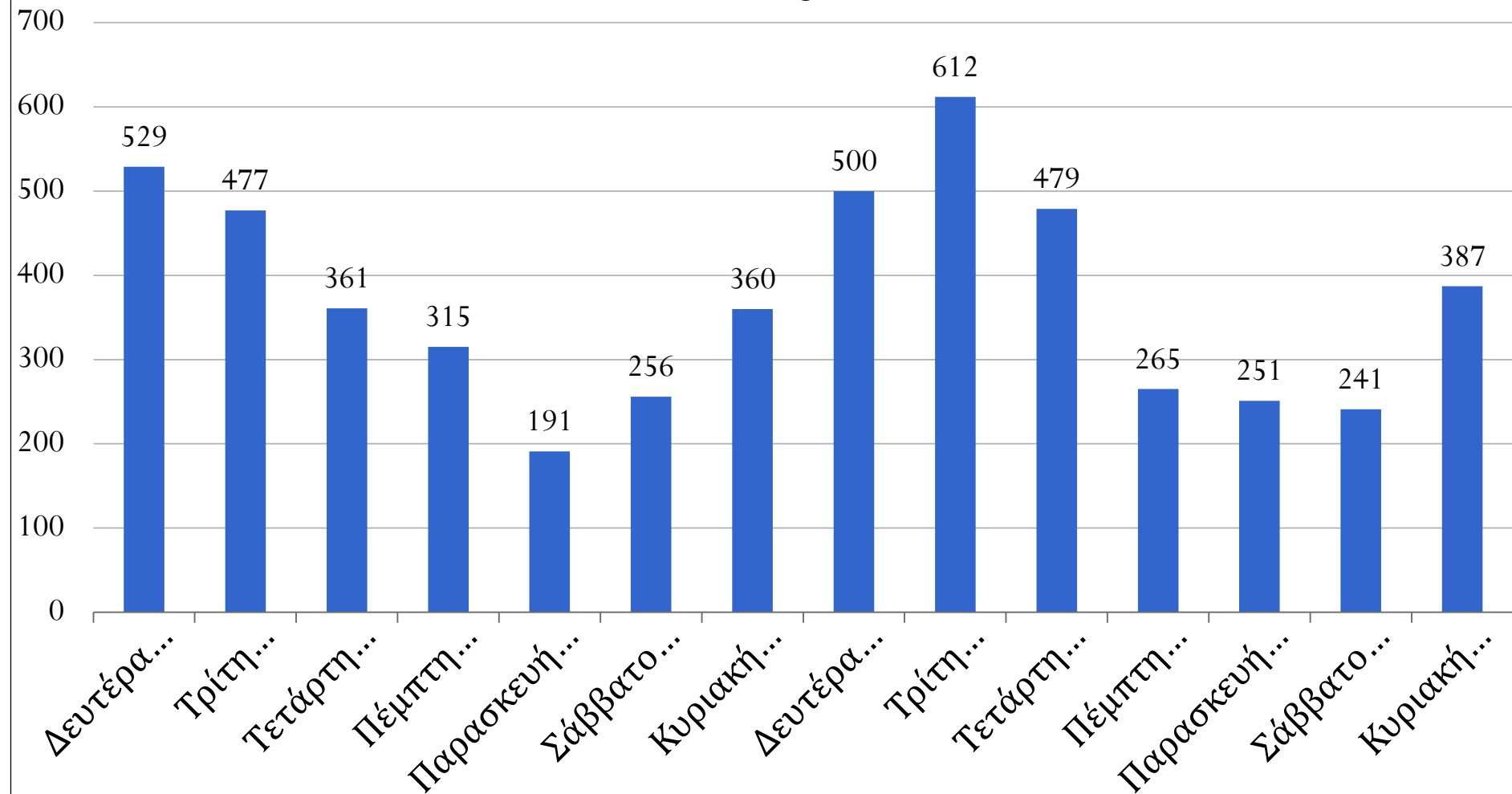
User Logins
